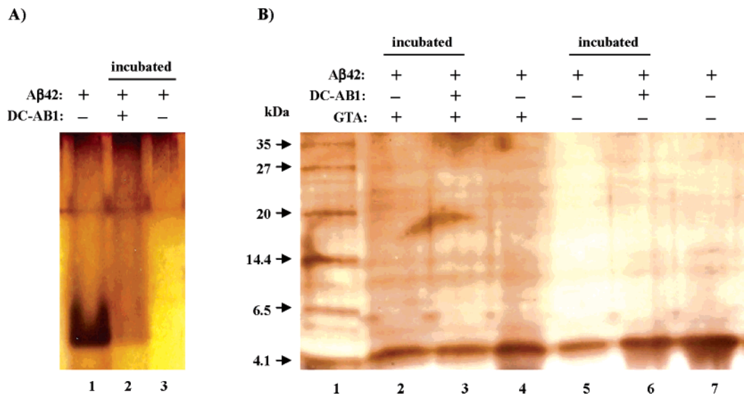
FIGURE 4: Native gel (10%) and 10% SDS–PAGE analysis of Aβ 1–42 incubated with or without DC-AB1. Equal amounts of Aβ 1–42 were loaded onto all of the lanes. The gels were run in a Tris/Glycine system and developed by the silver-stain method. (A) Native gel analysis of uncross-linked Aβ 1–42 samples. Lane 1: unincubated Aβ 1–42 ; lane 2: Aβ 1–42 incubated with DC-AB1; and lane 3: Aβ 1–42 incubated without DC-AB1. (B) SDS–PAGE analysis of cross-linked and uncross-linked Aβ 1–42 samples. Aβ 1–42 were cross-linked with 42 mM glutaraldehyde at room temperature for 20 min. Lane 1: marker; lane 2: cross-linked Aβ 1–42 , incubated without DC-AB1; lane 3: cross-linked Aβ 1–42 , incubated with DC-AB1; lane 4: cross-linked Aβ 1–42 , unincubated; lane 5: uncross-linked Aβ 1–42 , incubated without DC-AB1; lane 6: uncross-linked Aβ 1–42 , incubated with DC-AB1; and lane 7: uncross-linked Aβ 1–42 , unincubated.
