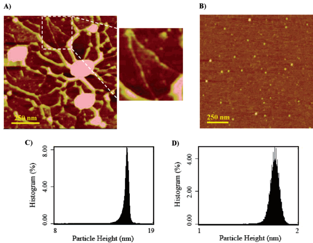
FIGURE 3: Morphological study of Aβ oligomers and fibrils by AFM experiment. (A) Aβ 1–42 (10 μM) forms protofibrils after 6 days of incubation at 37 °C in 20% TFE. (B) AFM scan image of a 10 μM Aβ 1–42 peptide sample incubated with 500 μM DC-AB1. (C) Statistical analysis of the particle height of oligomers and protofibrils in an Aβ 1–42 sample incubated without DC-AB1. (D) Statistical analysis of the particle height of aggregation species in an Aβ 1–42 sample incubated with DC-AB1.
