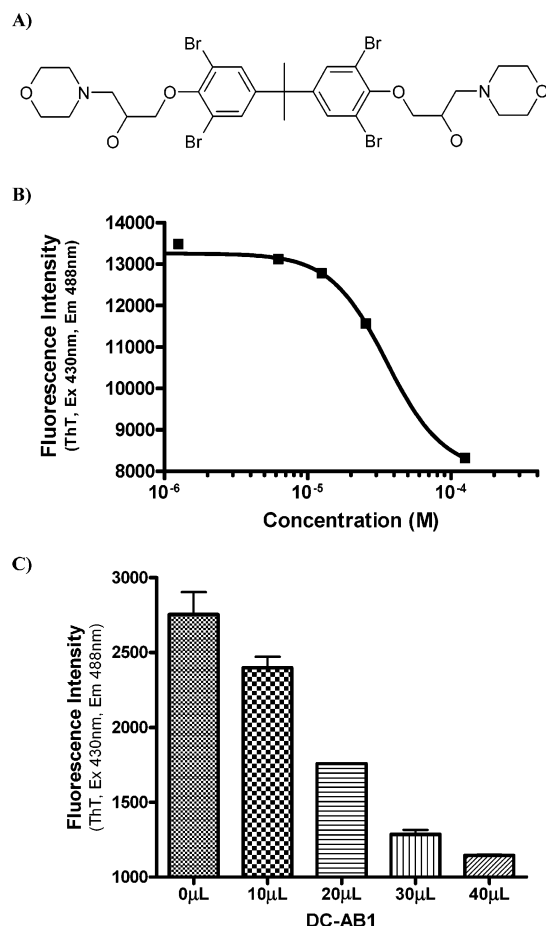
FIGURE 2: (A) Chemical structure of DC-AB1. (B) Concentration-dependent inhibition of DC-AB1 against Aβ fibrillation. (C) Amount of Aβ 1-42 fibrils formed after 20 h of incubation at 37 °C. Aβ 1-42 (2.5 μL of 200 μM) are incubated with 0, 10, 20, 30, and 40 μL of 10 mM DC-AB1, respectively. The decrease in fluorescence emission indicates the reduced amount of Aβ 1-42 fibrils formed, proving the inhibitory activity of DC-AB1.
